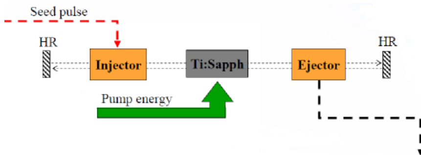
Figure 5.7: Regenerative amplifier seeded operation
