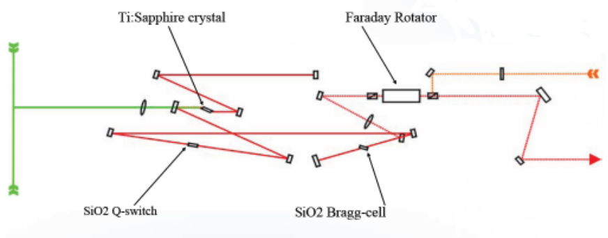
Figure 5.8: RegA 9050 Optical Scheme
