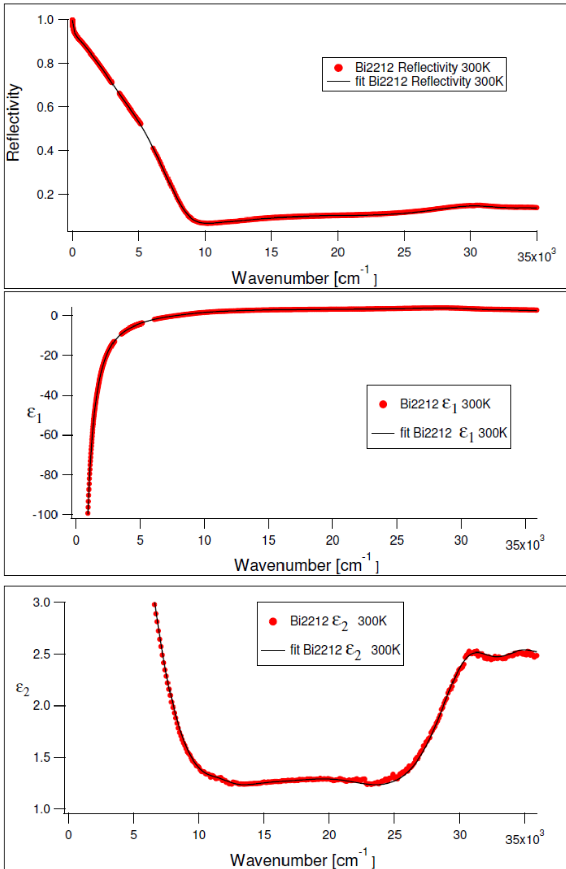
Figure 3.2: Y-Bi2212 Op 300 K: reflectivity, real and imaginary parts of the dielectric functions. Black lines are fit functions.
