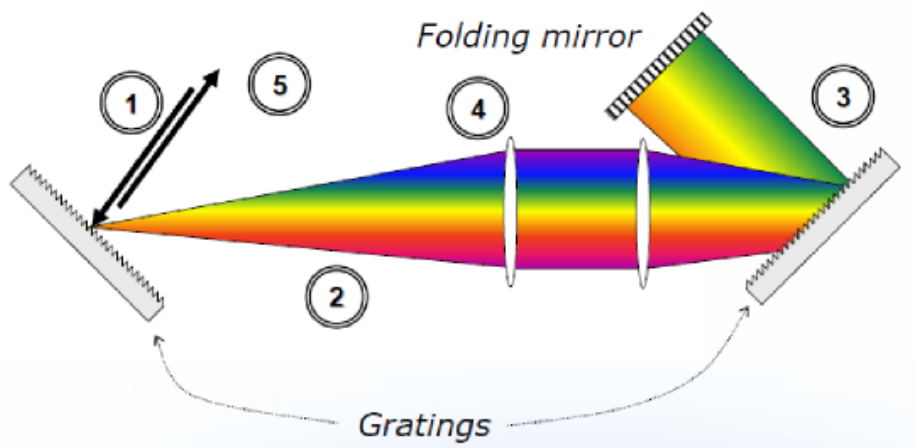
Figure 5.4: Stretching process of the pulse: 1) Input; 2) Positive dispersion; 3) Collimation of the beam; 4) Eliminating spatial chirp; 5) Output.
