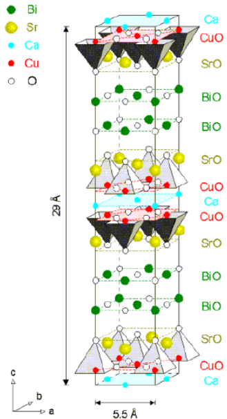
Figure 2.1: Bi2212 crystal structure - Crystal structure of Bi2212. Image from (39)
