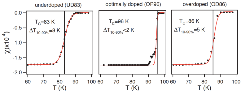
Figure 3.6: Samples characterization - Susceptibility measurements on the sample used in this work. The strong diamagnetic signal is associated with the superconducting state below T_C . The midpoint of the onset of superconductivity is chosen as the nominal T_C value, while the transition amplitude is calculated as the temperature interval between the 10% the 90% and drop of the susceptibility signal
