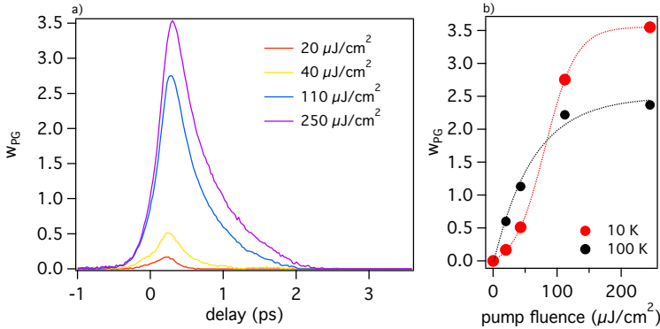
Figure 6.8: Pseudogap component dynamics - a) Dynamics of the weight of the pseudogap component w_{PG}(t) at different fluences. b) Peak intensity as a function of fluence.
