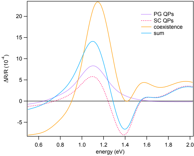
Figure 6.13: Differential model for SC and PG coexistence - Reflectivity variations obtained from the differential model for pseudogap quasi-particles 4.3.3, superconducting quasi-particles 4.3.4 (dashed lines) and a combination of the two perturbations (solid line) calculated including both effects for a differential model at 10 K. An algebraic sum of the two \Delta R/R signals of the two kinds of QPs is also shown.
