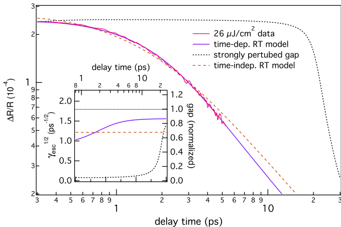
Figure 5.4: Application of time-dependent Rothwarf-Taylor model - |\Delta R/R| of the SCS at \Phi = 26 \mu \text{ J/cm}^2 and the corresponding fit (solid line) obtained with the numerical solutions of the time-dependent Rothwarf-Taylor equations, (5.1) and (5.2), considering a d-wave gap symmetry. The a optimal value is (1.0 \pm 0.2) \times 10^{-20} \text{ cm}^3 . For comparison we also show the fits when the parameter a is fixed to the values a = 2.45 \times 10^{-20} \text{ cm}^3 (short-dashed) and a = 0 (long-dashed), which is equivalent to the time-independent RT model. In the inset we show the corresponding function (\gamma_{esc}(t))^{\frac{1}{2\alpha}} , which is proportional to the non-equilibrium superconducting gap \Delta(t) (5.3). We normalized the gap to the low-fluence value (See Sec. 2.3.1).
