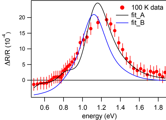
Figure 4.12: Fit of the 100 K data with the differential model - Principal component of the optical response at 100 K and the corresponding fit obtained with the differential EDM (see text). In fit A the spectral weight of the Drude term and of mid-infrared peaks are used as free parameters. In fit B the spectral weight of the Drude term and the low-energy peak of the glue function are used as free parameters.
