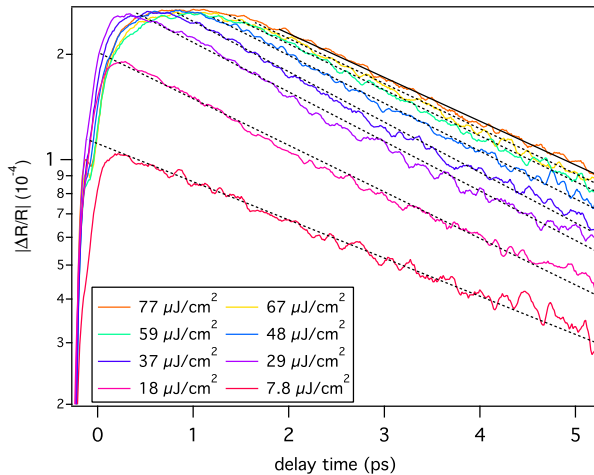
Figure 5.3: Relaxation of superconducting signal at high fluence - We report the |\Delta R/R| traces in logarithmic scale at several pump fluences at T = 10 K, where the exponential A component has been subtracted. The dashed lines represent the exponential fit of the decay. The solid line refers to the curve at \Phi = 77 \mu\text{J}/\text{cm}^2 .
