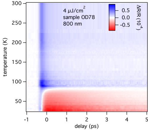
Figure 4.14: Temperature dependence of the interband spectral weight - Temperature-time matrix of the \Delta R/R signal on the OD78 sample at 1.55 eV at a pump fluence of 4 \mu\text{J}/\text{cm}^2
